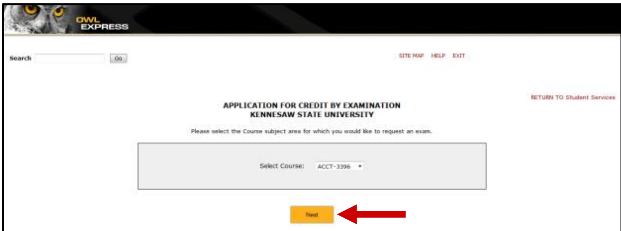
Figure 5 – Click Next
